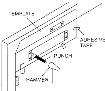
TAPPING SCREW (FOR WOODEN DOOR)
