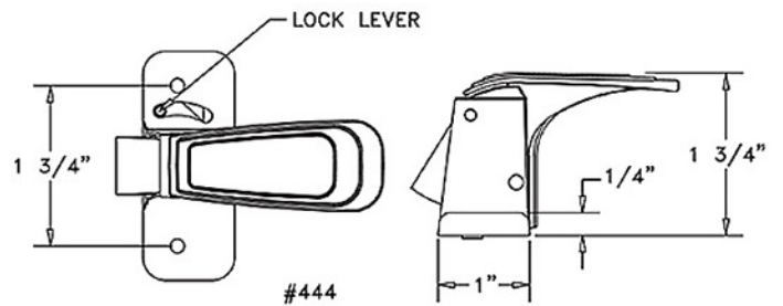
Interior Latch for V_444 Push Button Latches
